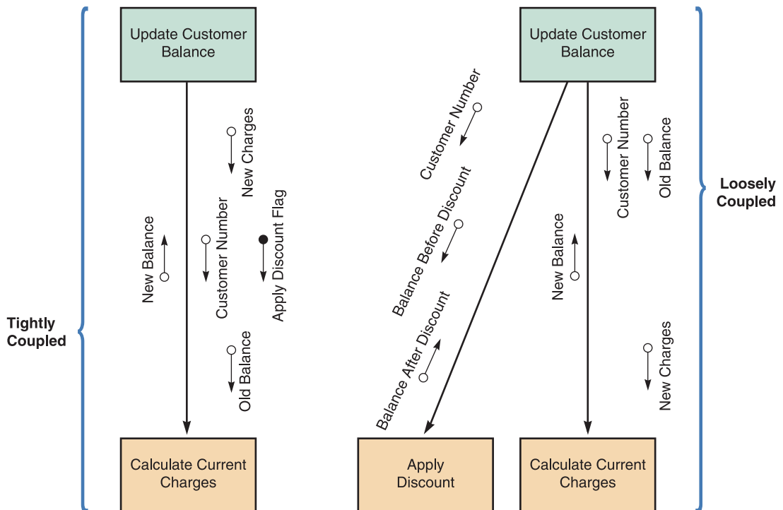
FIGURE 11-14 An example of tightly coupled and loosely coupled structure charts.
