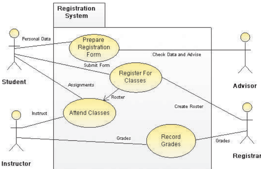
FIGURE 4-13 This Visible Analyst use case diagram shows a student records system. Source: Visible Systems Corporation.
