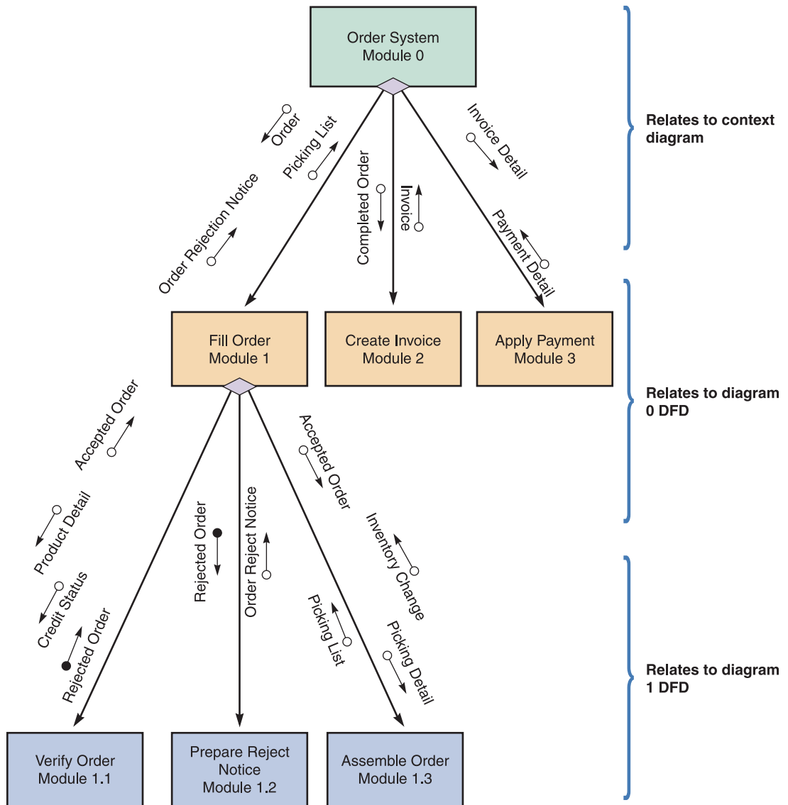
FIGURE 11-15 A structure chart based on the order system DFDs in Chapter 5. The three-level structure chart relates to the three DFD levels.
