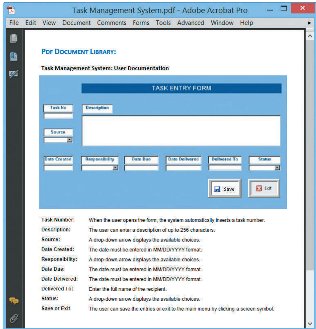
FIGURE 11-24 A sample page from a user manual. The instructions explain how to add a new task to the system.
