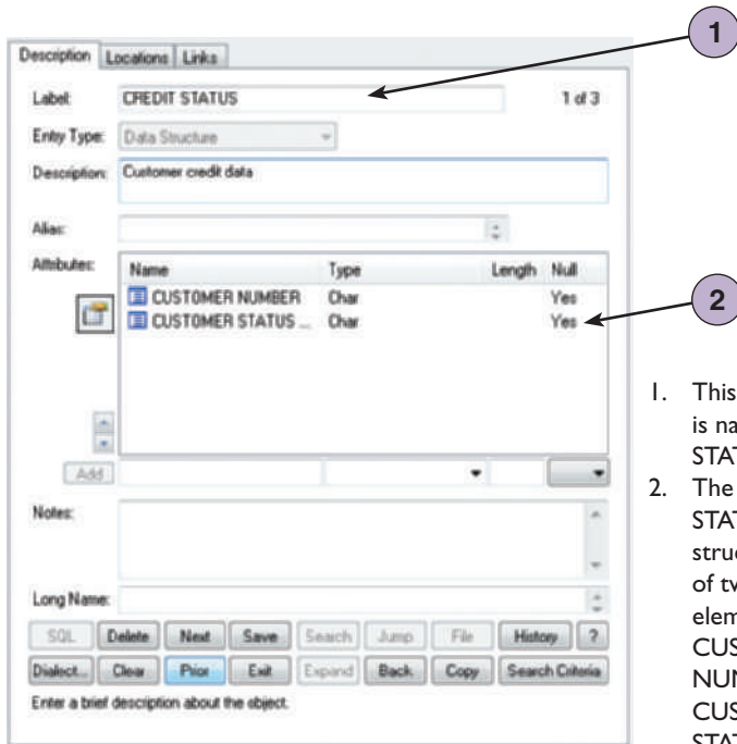
FIGURE 5-23 A Visible Analyst screen that documents a record, or data structure, named CREDIT STATUS
