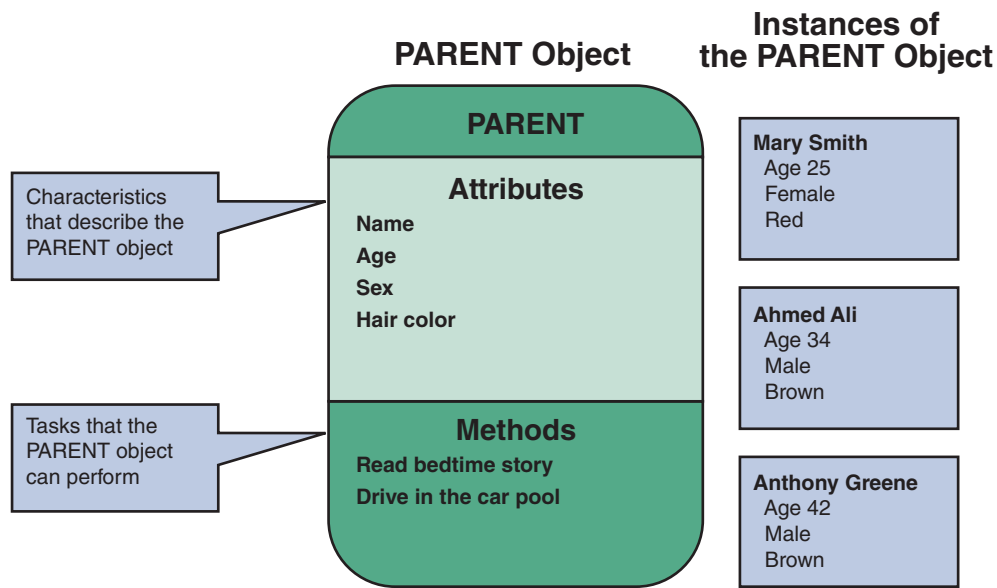
FIGURE 6-2 The PARENT object has four attributes and two methods. Mary Smith, Ahmed Ali, and Anthony Greene are instances of the PARENT object.
